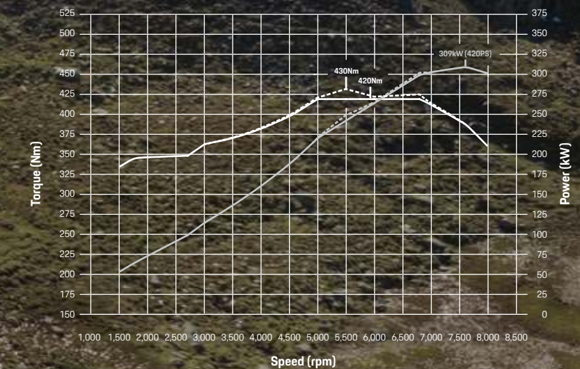
718 Spyder: 309kW (420PS) at 7,600rpm — 6-speed manual transmission: 420Nm between 5,000 and 6,800rpm - - - - Porsche Doppelkupplungsgetriebe (PDK): 430Nm at 5,500rpm
