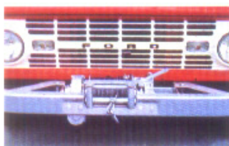
Front-Mounted Winch with 150 feet of 3/16-inch cable is power take-off driven.
